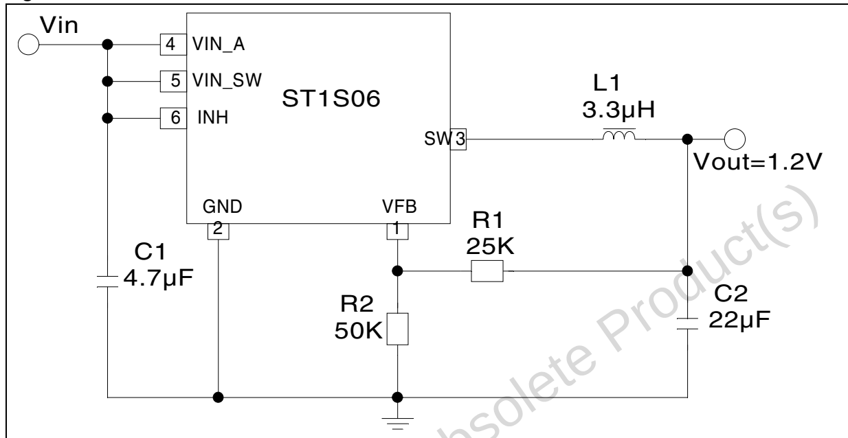
Figure 1. Circuit schematic
